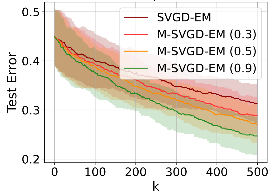
N = 20 particles
