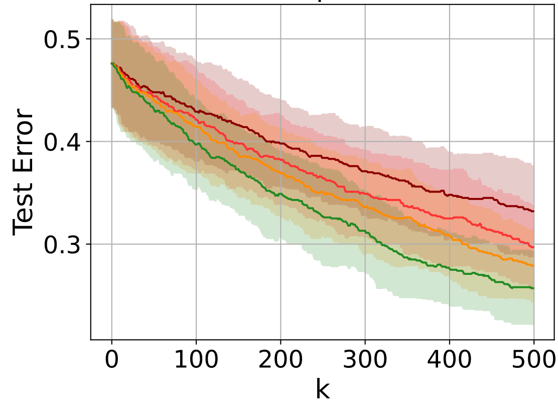
N = 10 particles
